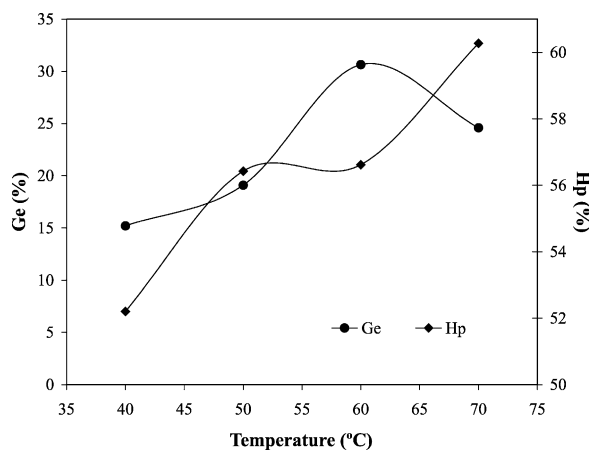
Fig. 5. Effect of varying the temperature on the grafting of PMMA onto wood-fiber. Experiments were carried out using an overall concentration of 0.024 \text{ mol l}^{-1} at a molar ratio of 0.2. The surfactant concentration was 2.0 \text{ mmol l}^{-1} in all cases.
