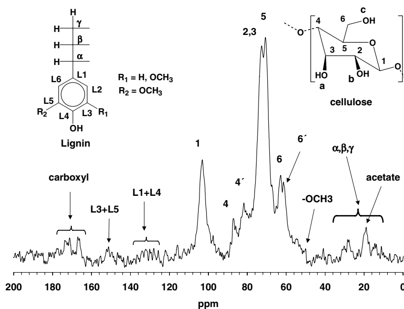
Fig. 3. CP/MAS ^{13}\text{C} NMR spectrum for blue agave fiber before modification.
